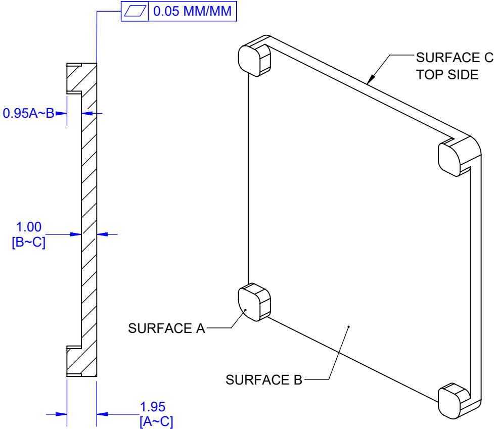
SECTION E-E SCALE 4 : 1
