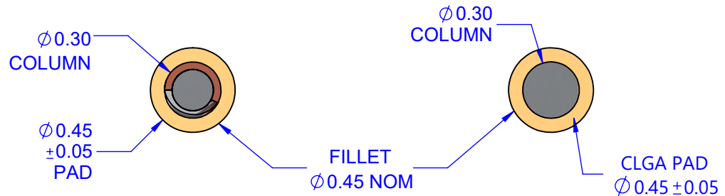
SECTION C-C SCALE 35 : 1
