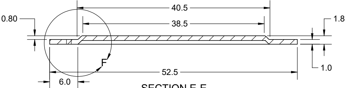
SECTION E-E
