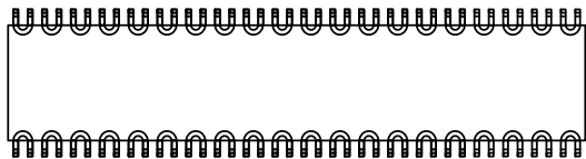
80L DWG 128003
