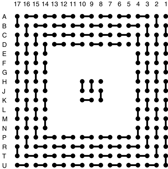
BALL VIEW
