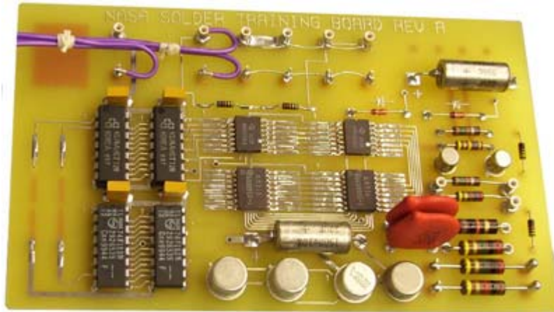
Photo shown after assembly. PWB Size: 4.0" x 5.5" (100 x 140mm)
