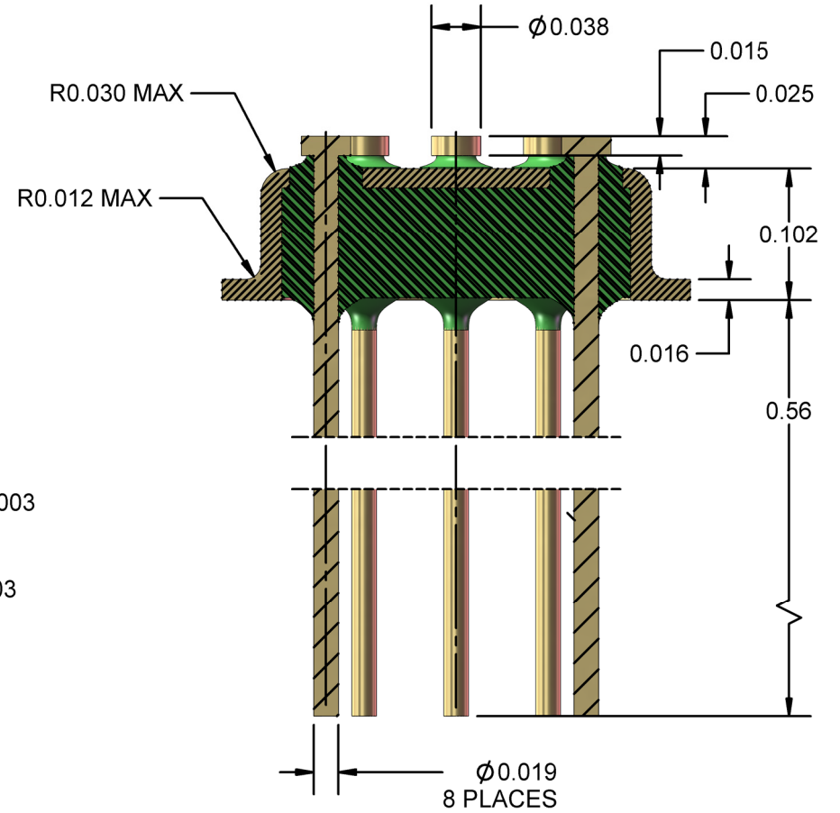
SECTION A-A SCALE 7.5 : 1
