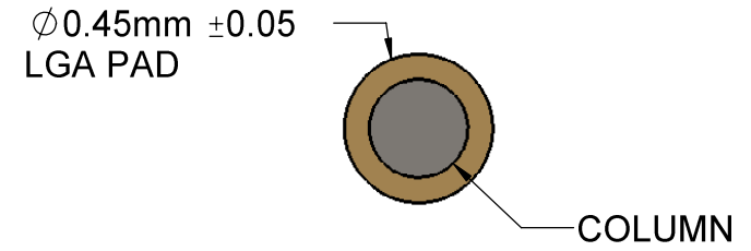
LGA - LAND GRID ARRAY PAD PLATING Ni-Au
