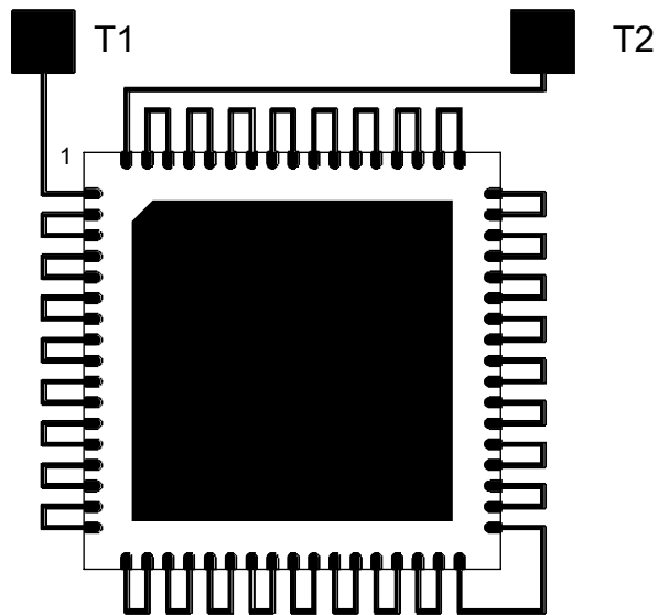
RECOMMENDED PCB PADS
