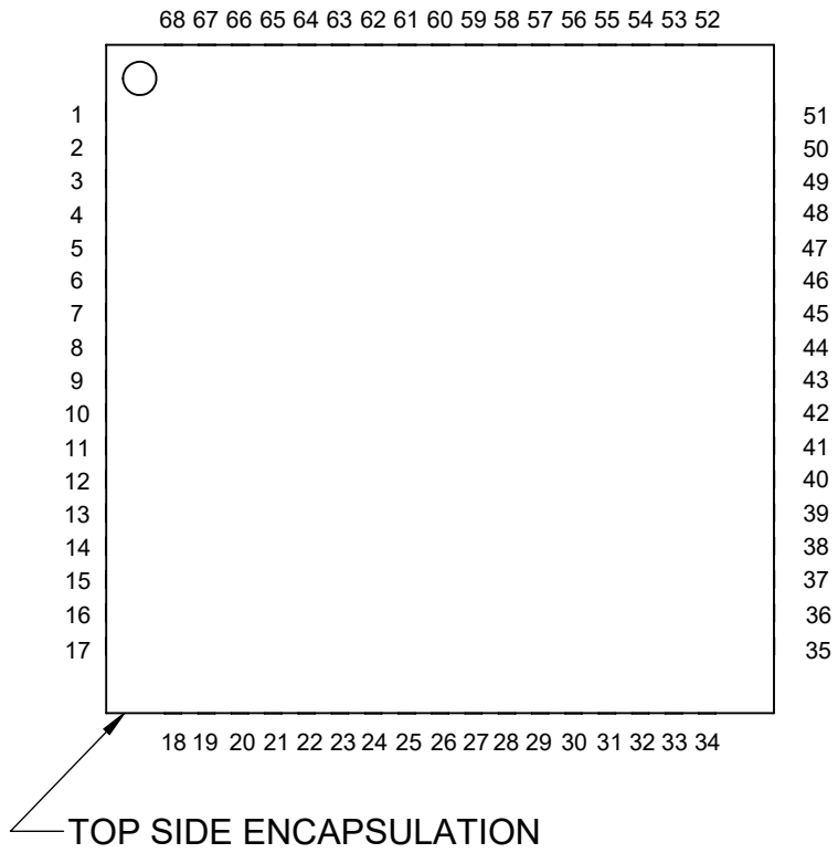
TOP VIEW
