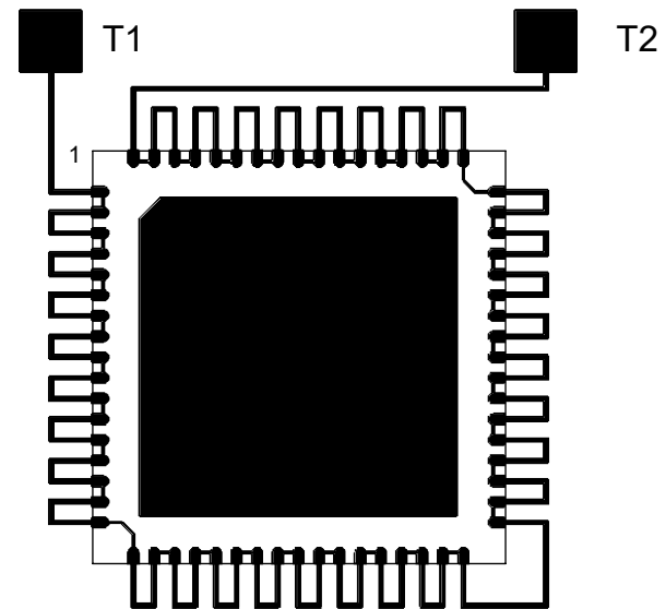
AFTER MOUNTING ON PCB
