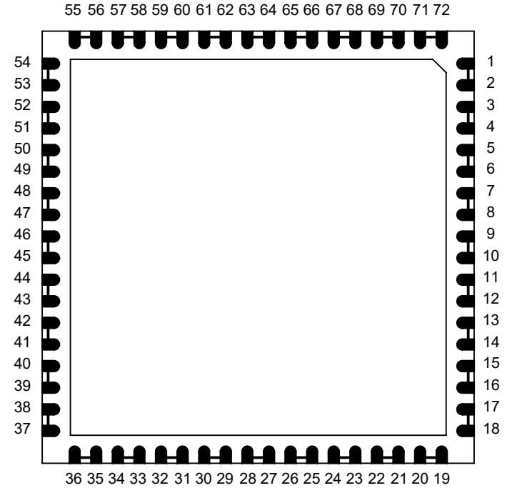
BOTTOM VIEW
