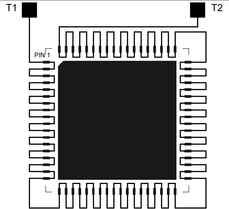
AFTER MOUNTING ON PCB
