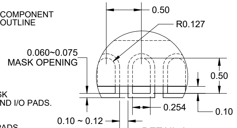
DETAIL A SCALE 30 : 1
