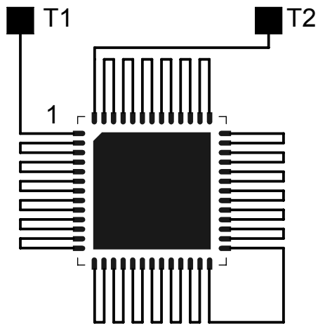
RECOMMENDED PCB PADS
