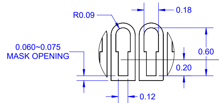
DETAIL A SCALE 35 : 1
