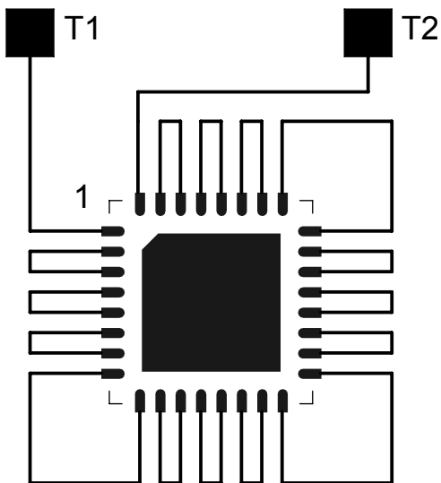
RECOMMENDED PCB PADS
