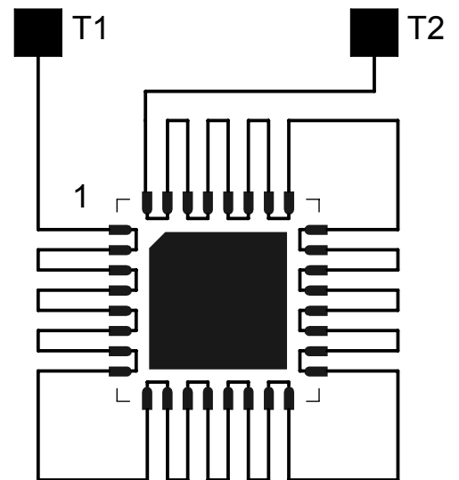
AFTER MOUNTING ON PCB
