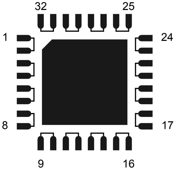
QFN DAISY CHAIN INTERNAL CONNECTIONS
