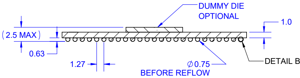
SECTION A-A SCALE 2.5 : 1
