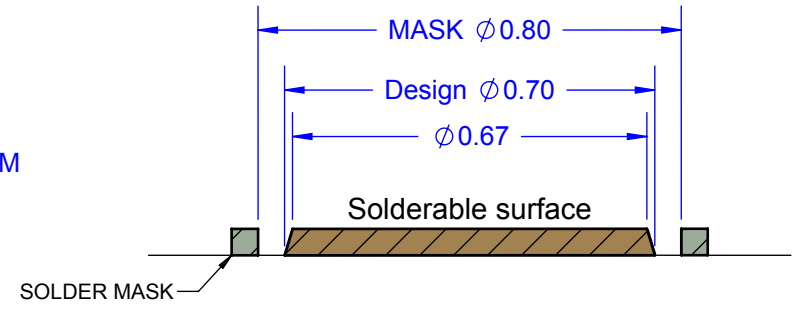
Section B-B
