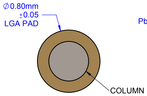
LGA - LAND GRID ARRAY PAD PLATING Ni-Au
