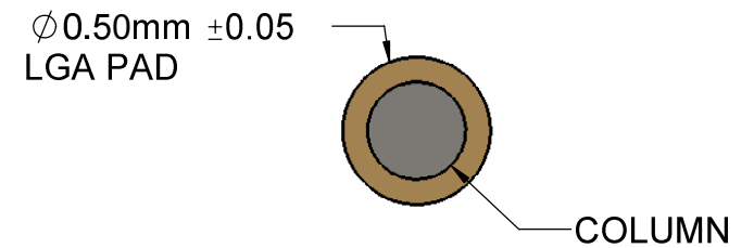
LGA - LAND GRID ARRAY PAD PLATING Ni-Au
