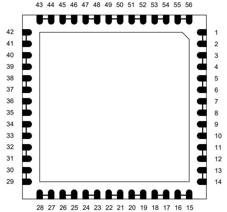
BOTTOM VIEW
