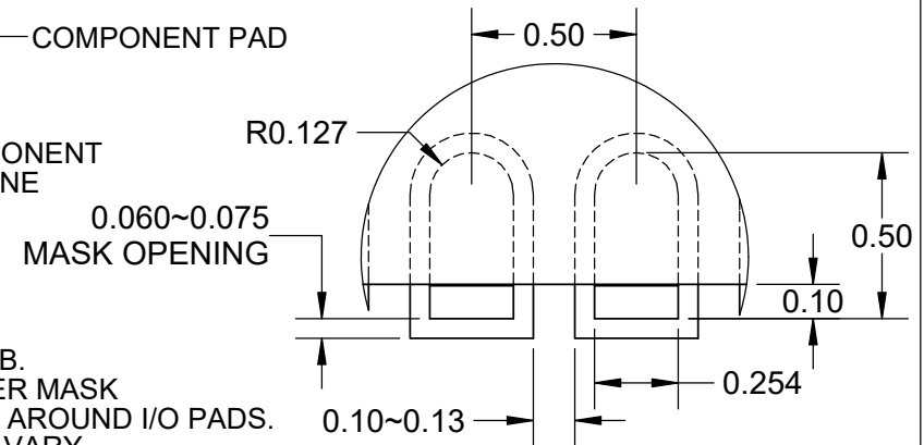
DETAIL A SCALE 40 : 1
