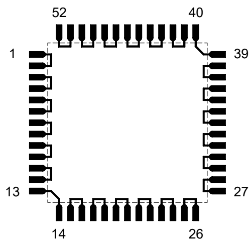
COMPONENT VIEW FROM TOP
