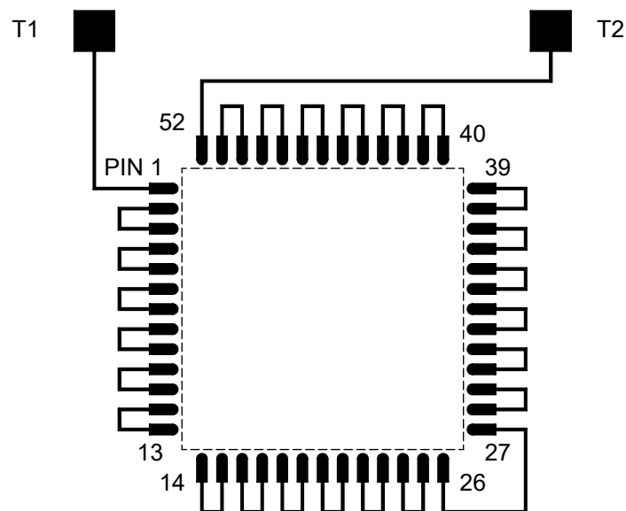
RECOMMENDED PCB PADS
