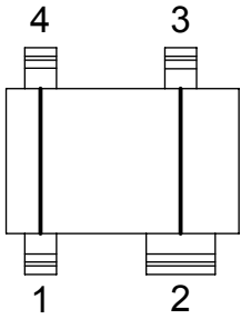
SOT343-DC1423
