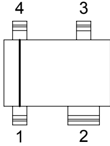
SOT343-DC14
