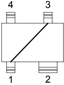
SOT343-DC13
