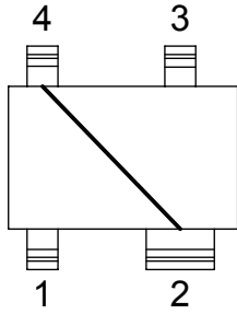
SOT343-DC42
