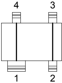
SOT143-DC1423
