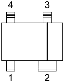
SOT343-DC22
