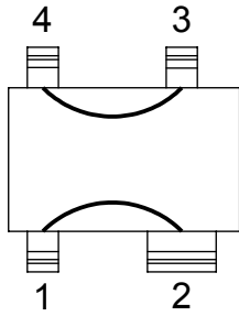
SOT343-DC1234
