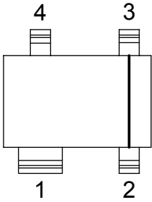
SOT143-DC22
