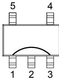
SOT25 - DC31 DWG 120531
