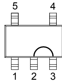
SOT353 - DC32 DWG 120532
