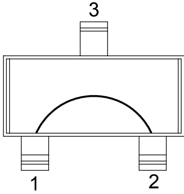
SOT523 - DC12 DWG 120312
