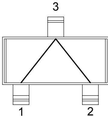
SOT523 - DC123 DWG 120123
