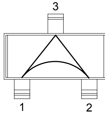
SOT523 - DC1231 DWG 121231
