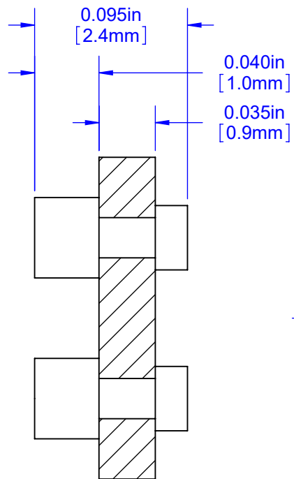
SECTION B-B
