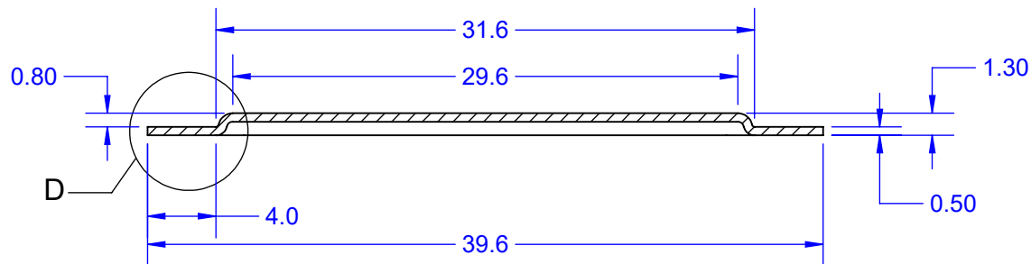
SECTION C-C SCALE 2.5 : 1
