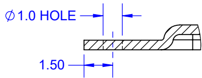
DETAIL B SCALE 5 : 1
