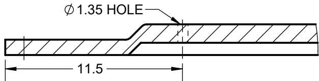
DETAIL F SCALE 4 : 1
