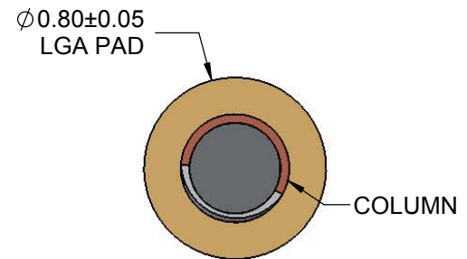
LGA - LAND GRID ARRAY PAD PLATING Ni-Au
