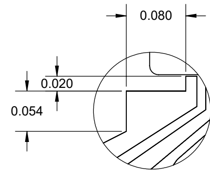
DETAIL B SCALE 8 : 1 NO.1 INDEX MARK
