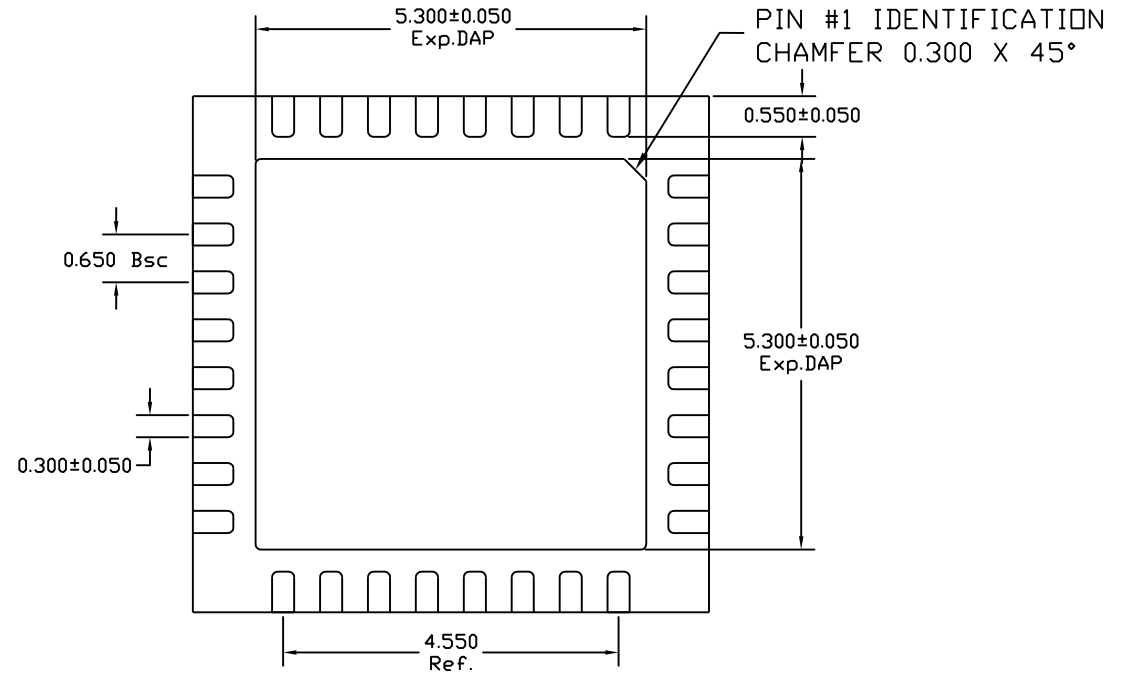
BOTTOM VIEW
