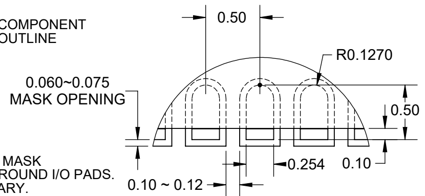
DETAIL A SCALE 28 : 1
