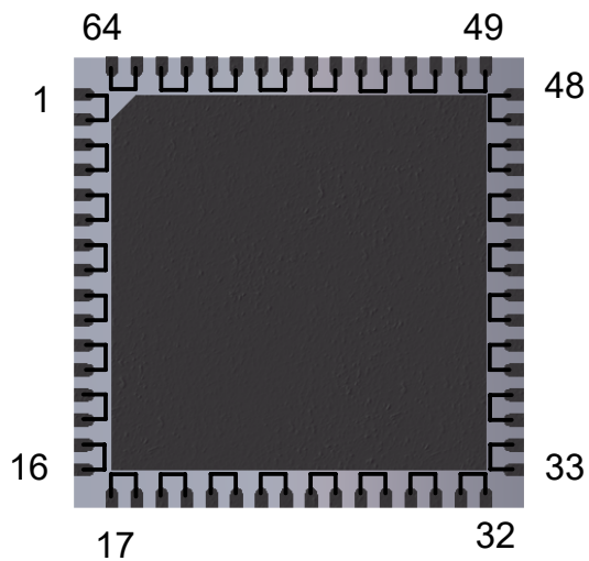
VIEW FROM TOP
