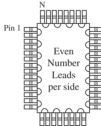
RECTANGLE BODY
