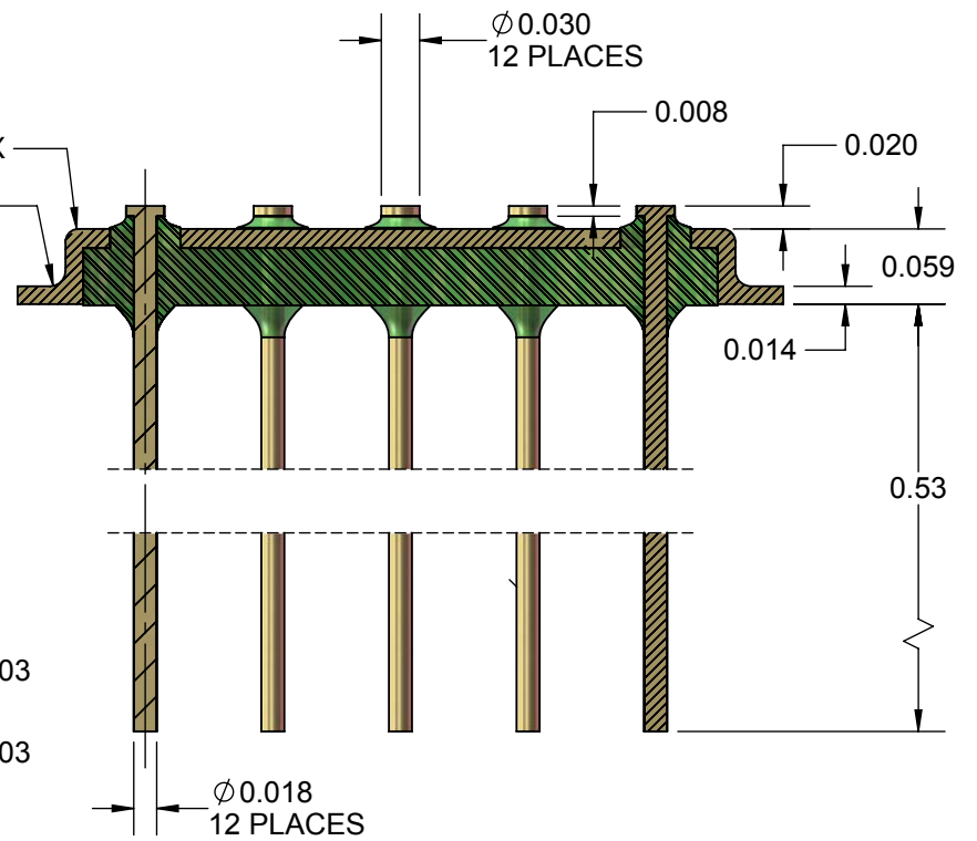
SECTION A-A SCALE 6:1
