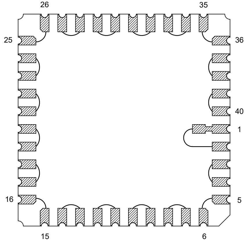
BOTTOM VIEW
