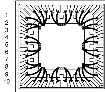
11 13 15 17 19 12 14 16 18 20 QFN40W.4-DCW25402 40L - 5X5mm
