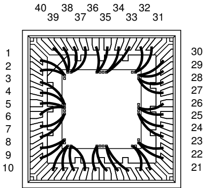
11 13 15 17 19 12 14 16 18 20 QFN40W.4-DCW25401 40L - 5X5mm
