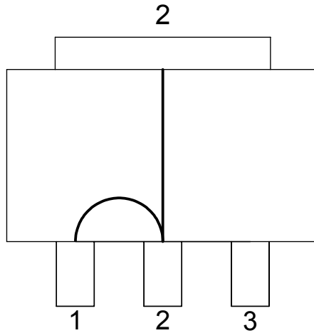
SOT223 - DC124 124124
